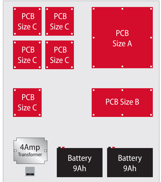
Hinged Expansion Plate layout option Purchased separately 999027
